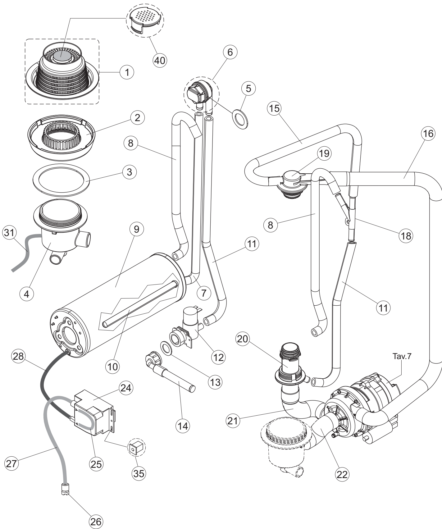
Drain Pump
